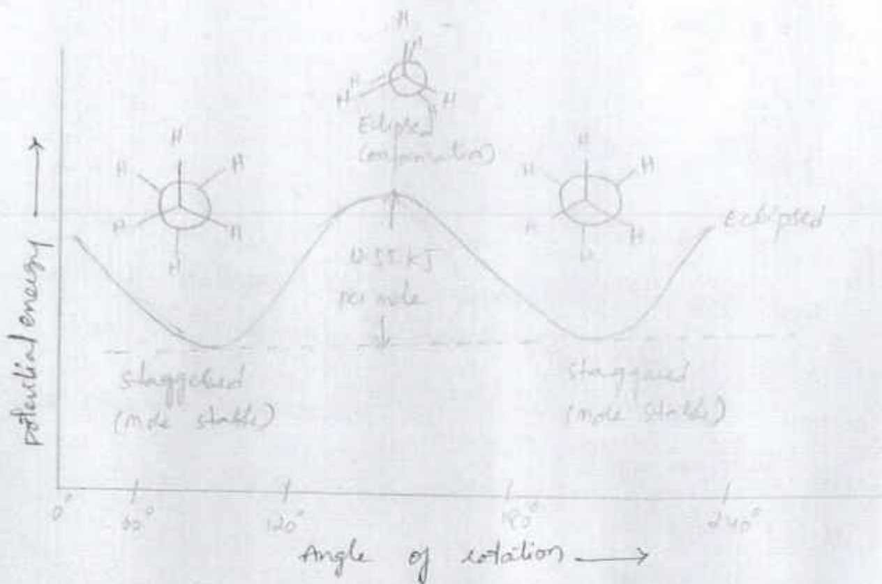
potential energy change during the rotation about C-C bond in ethane.
