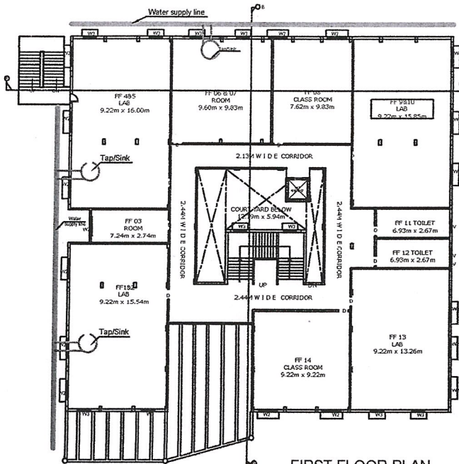
FIRST FLOOR PLAN MORTGAGE AREA
